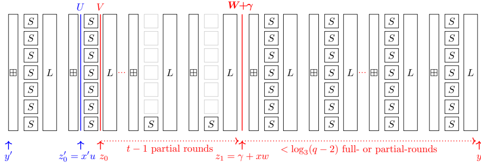
Figure 10: Zero-sum distinguisher against POSEIDON and STARKAD covering (2 + 4) full rounds and all partial rounds.
